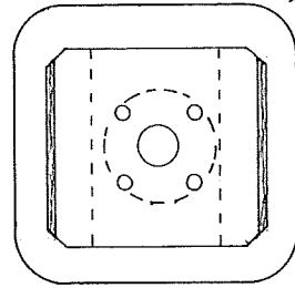
Front view of Motor Mount
